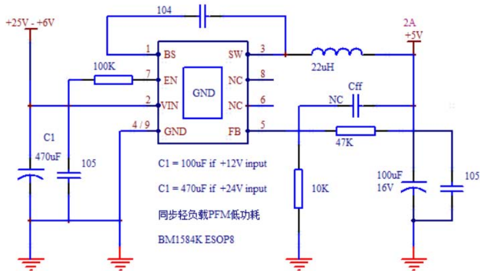
Figure 2. BM1584 K 或 B M 1 5 8 4 D Application Circuit
